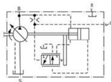
恒功率变量LV Constant power control
