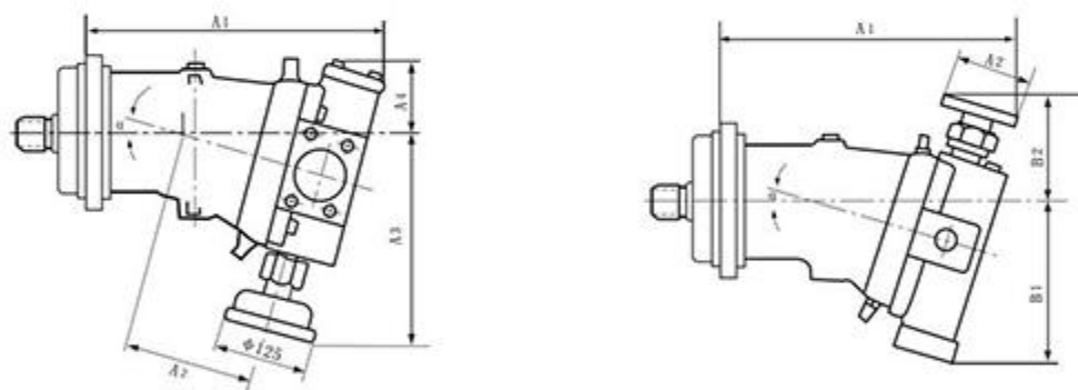
手轮朝下 handwheel downwards
